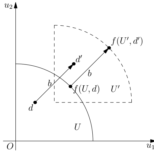
Figure 22.3: Independence of utility origins.
