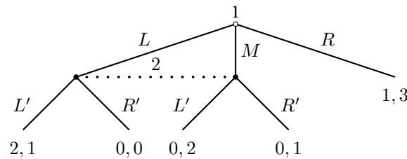
Figure 13.11: Motivation of perfect Bayesian equilibrium
